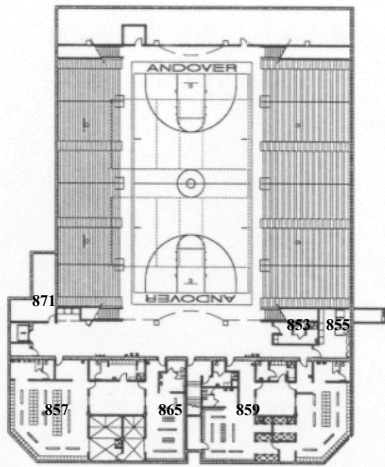
LOWER LEVEL PLAN
